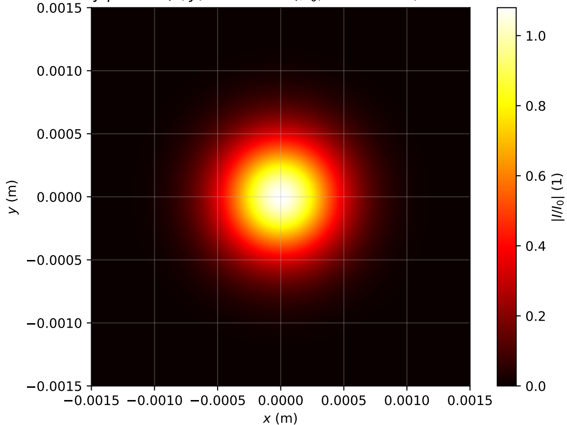
Intensity profile I(x, y, z = 0.398m)/I_0 , P_{in}=0.8P_{cr} , artificial time
